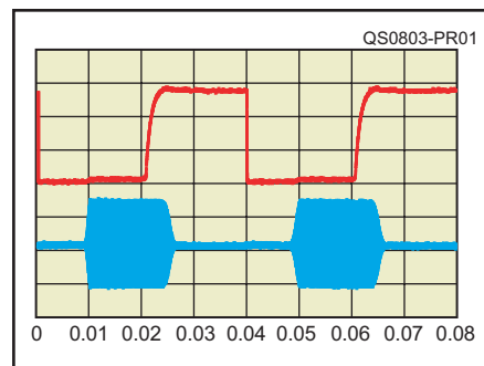
Figure 1 — CW keying waveform for the Yaesu FT-950 showing the first two dits in full-break-in (QSK) mode using external keying. Equivalent keying speed is 60 WPM. The upper trace is the actual key closure; the lower trace is the RF envelope. (Note that the first key closure starts at the left edge of the figure.) Horizontal divisions are 10 ms. The transceiver was being operated at 100 W output at 14.2 MHz.
