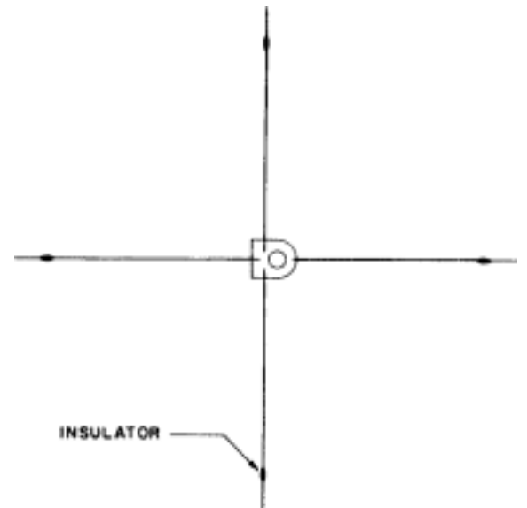
ALTERNATE SYSTEM ALL RADIALS 33' (10.058 m) FROM BOLT TO INSULATOR
