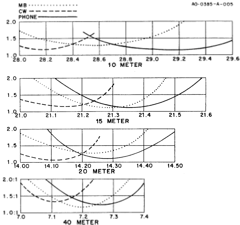
Figure 7 VSWR Curves
