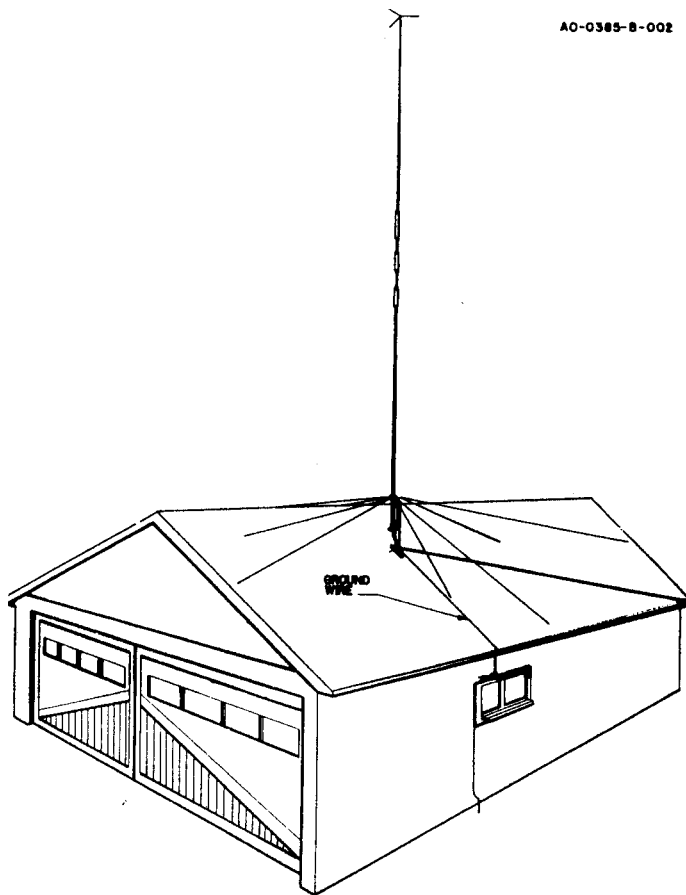
Figure 6 Completed Installation of 14AVO/WB-S
