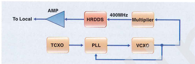
Local Oscillator block diagram
