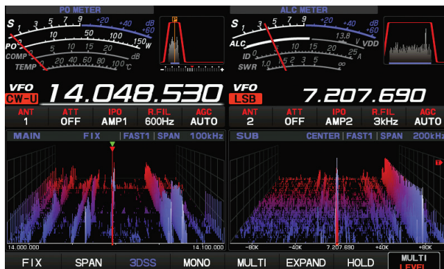
Figure 3 — Same as Figure 2, except a second spectrum view of the sub receiver display has been added to the right of the first spectrum display for the main receiver. Note that the second receiver is on a different band and using a different mode, bandwidth, and antenna. Either receiver can be tuned anywhere within the FTDX101D's tuning range, independent of the other receiver's settings. The two displays can also be one above the other, if you prefer — lots of flexibility available.
