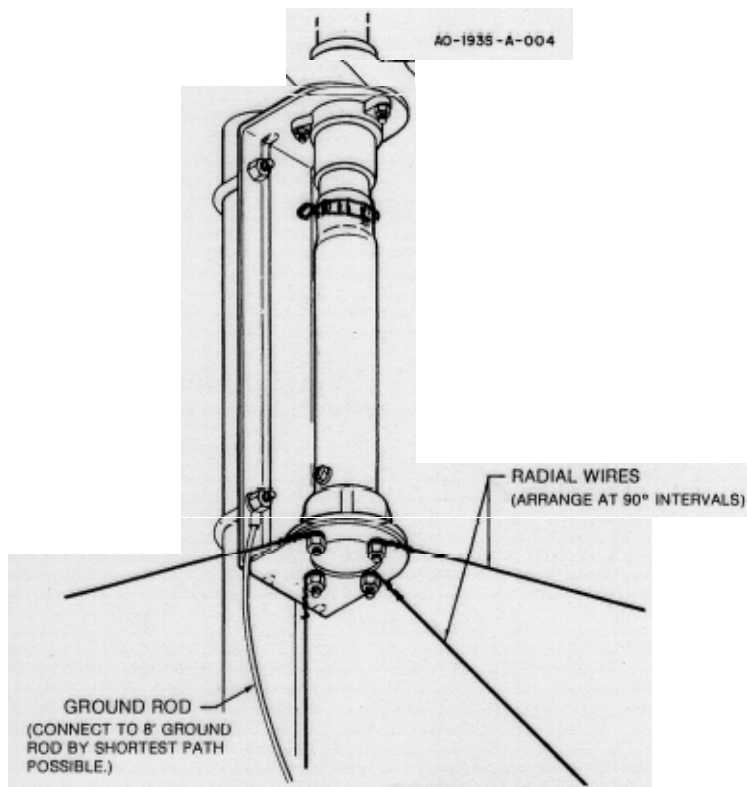
Figure 5 Method of Attaching Radial Wires to Base
